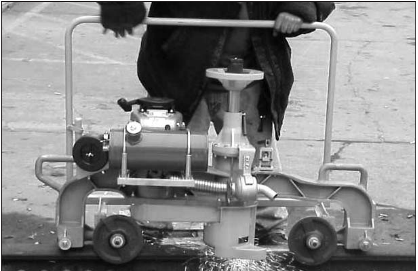
The Profile Grinder restores the true contour on continuous welded rail
