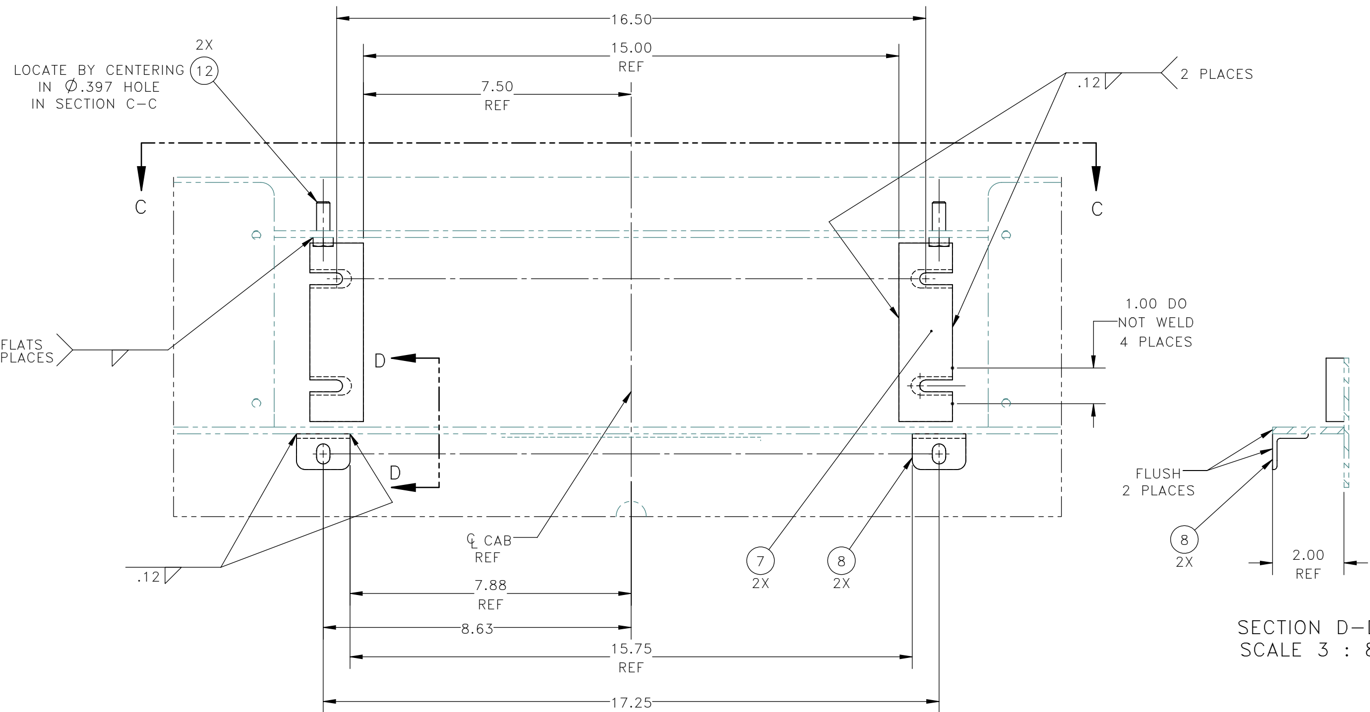
DETAIL B SCALE 3 : 8
