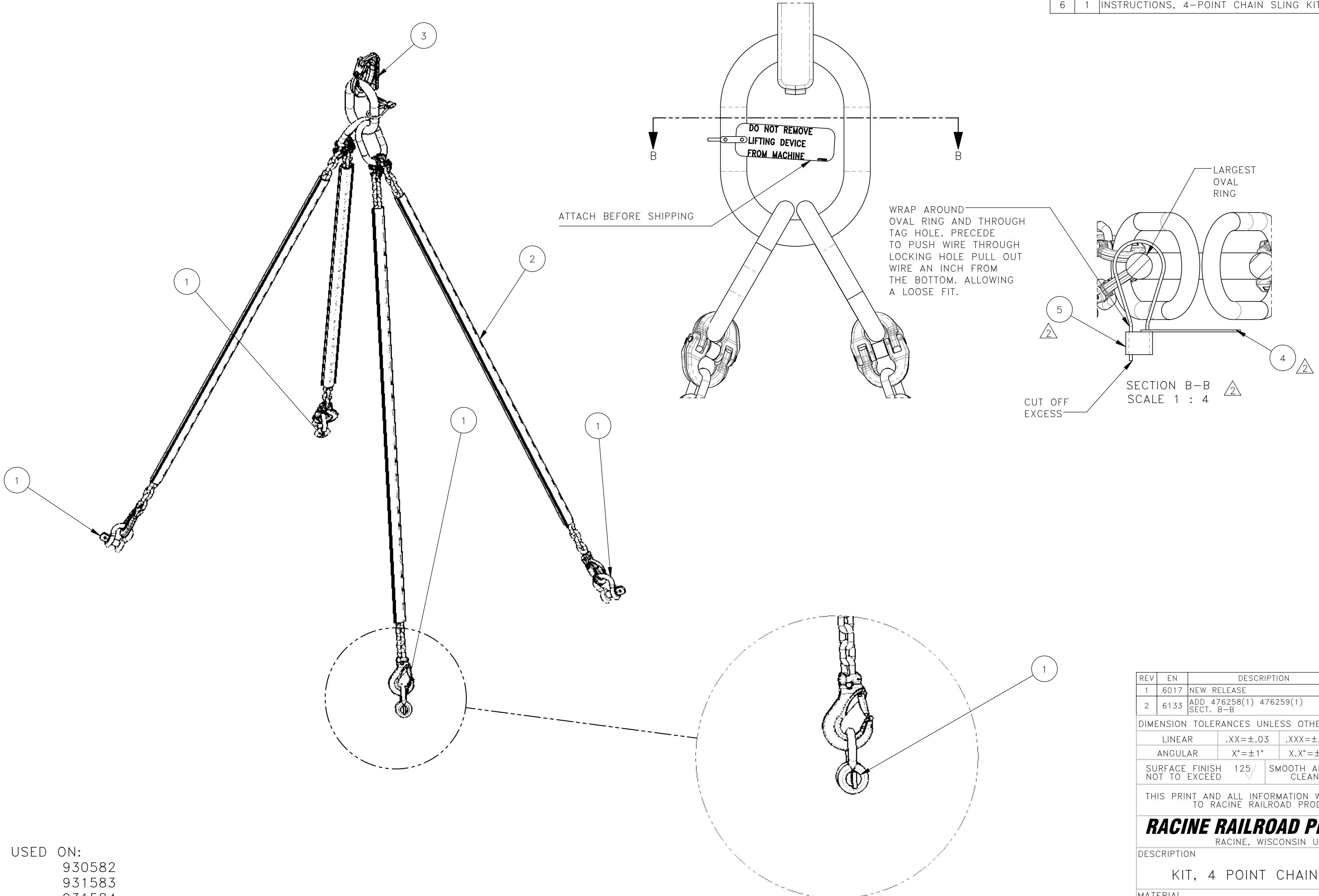
DETAIL A 4 PLACES SCALE 1 : 7
