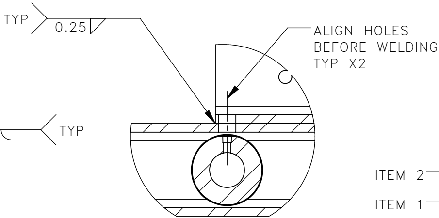
DETAIL C SCALE 1 : 4
