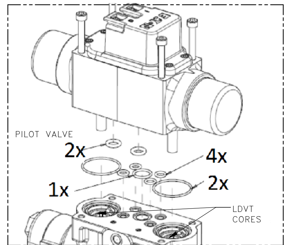
FIG 2.2 CMA200 PV SEALS ** PER WORK SECTION
