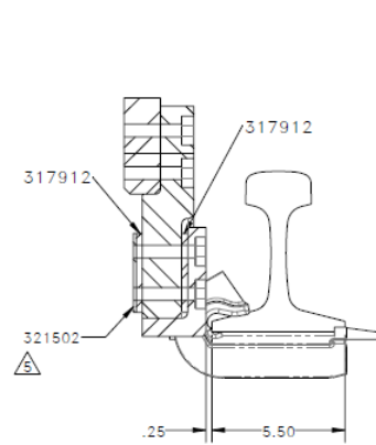
SECTION C-C SCALE 1 : 4
