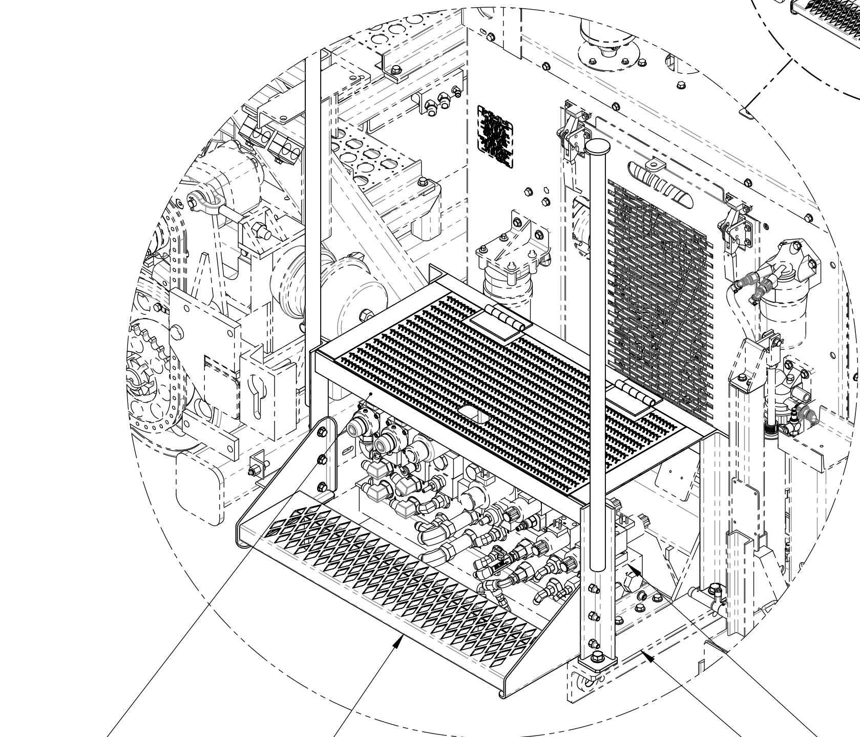
DETAIL A SCALE 1 : 8
